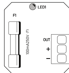
Figure 3 Layout of the electrical connection
